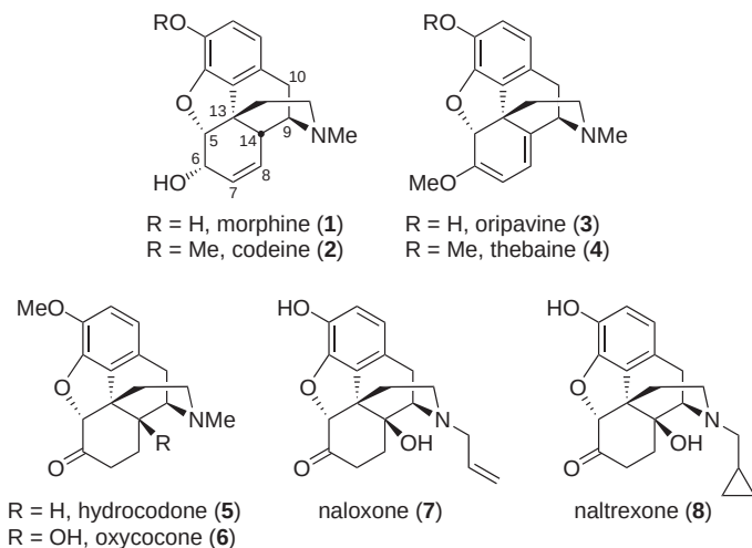
FIG. 1 Morphine alkaloids and some of their semisynthetic derivatives
