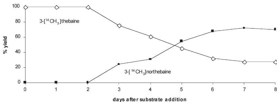
FIG. 5 Conversion of 3-[ ^{14}\text{CH}_3 ]thebaine to 3-[ ^{14}\text{CH}_3 ]northebaine by C. echinulata cultures
